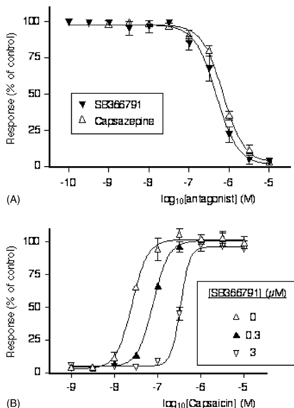
Fig. 2. SB366791 is a competitive antagonist at rat VR1. (A) Intracellular \text{Ca}^{2+} concentration was monitored using Fluo-3 in rat vanilloid VR1 receptor-HEK293 cells before and after the addition of capsaicin (100 nM), in the presence or absence of Caps (1 nM–10 \mu M) or SB366791 (0.1 nM–10 \mu M). (B) Effects of 0.3 and 3 \mu M SB366791 upon the concentration response curves to capsaicin. Data are mean \pm SEM where N = 5 .
