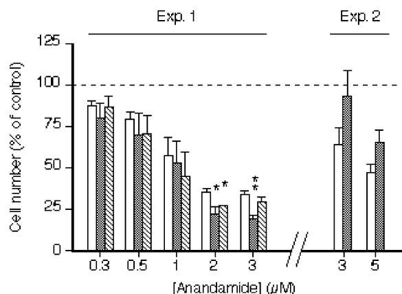
Fig. 5. Effect of palmitoyltri- and -ethylamides upon the antiproliferative effects of anandamide. Anandamide was administered daily for 4 days in the absence (unfilled columns) or presence of either palmitoyltri- or -ethylamide (filled and hatched columns, added concentration: 30 \mu M) and cell proliferation was measured on day 5. Shown are means \pm SEM, N = 3 for two separate experiments. * P < 0.05 , ** P < 0.01 vs. the corresponding value in the absence of palmitoyltri- or -ethylamide (two-tailed t -test).
