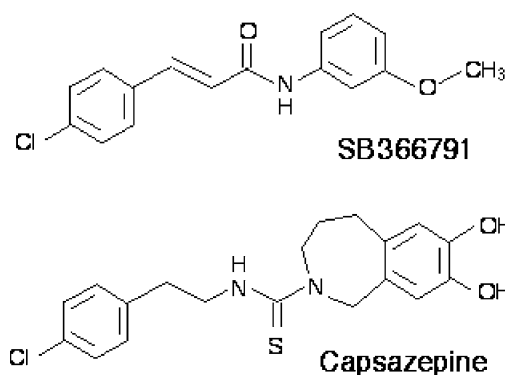
Fig. 1. Structures of capsazepine (Caps) and SB366791.
